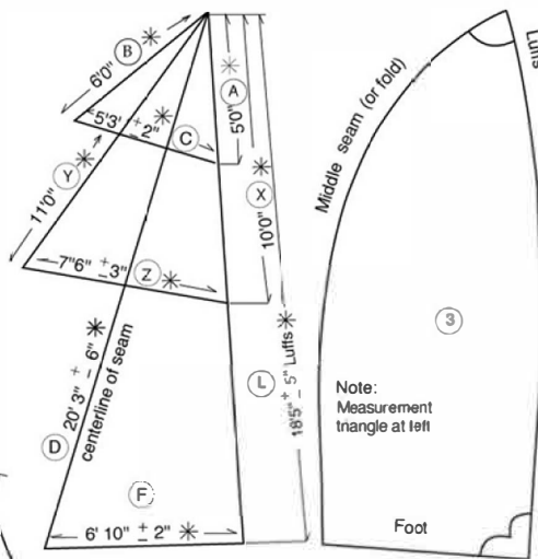
(Measurement Pattern of Spinnaker Folded Along Center Seam or Fold)
